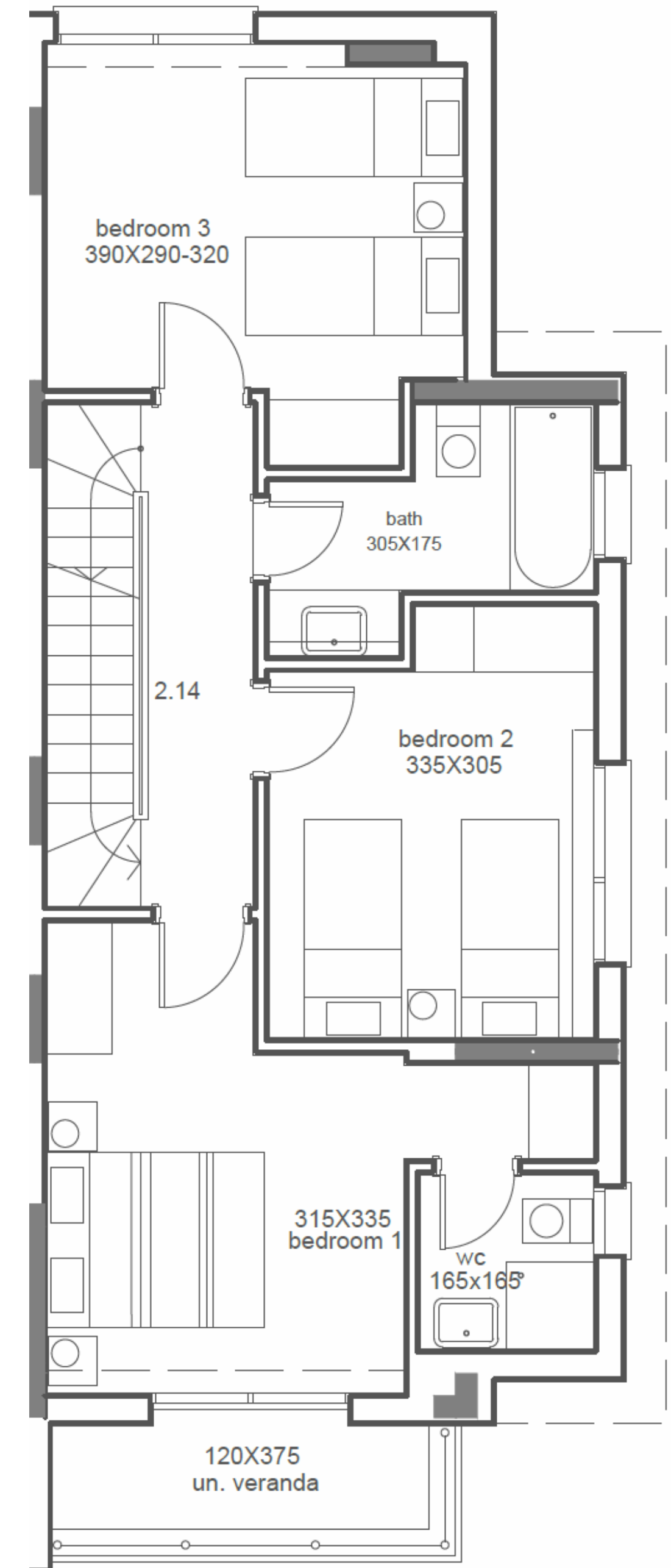
FIRST FLOOR
