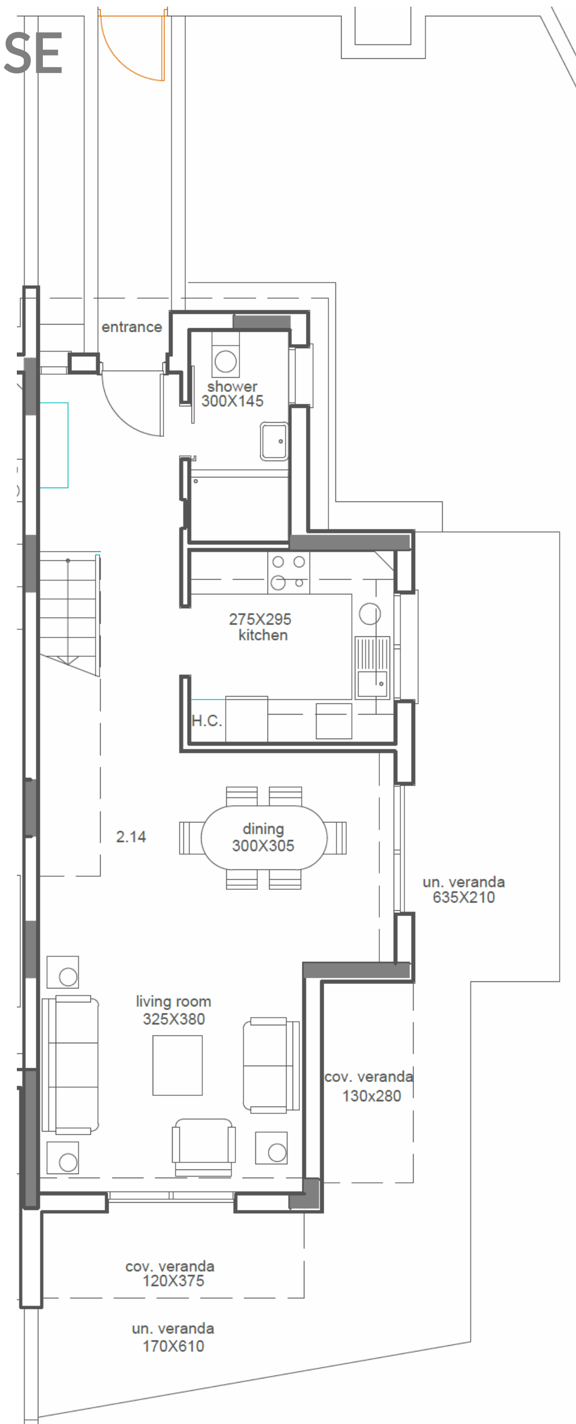
FIRST FLOOR
